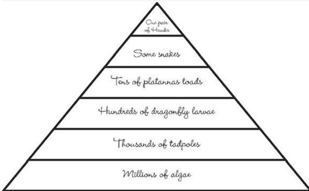
Pyramid of numbers for a local pond
